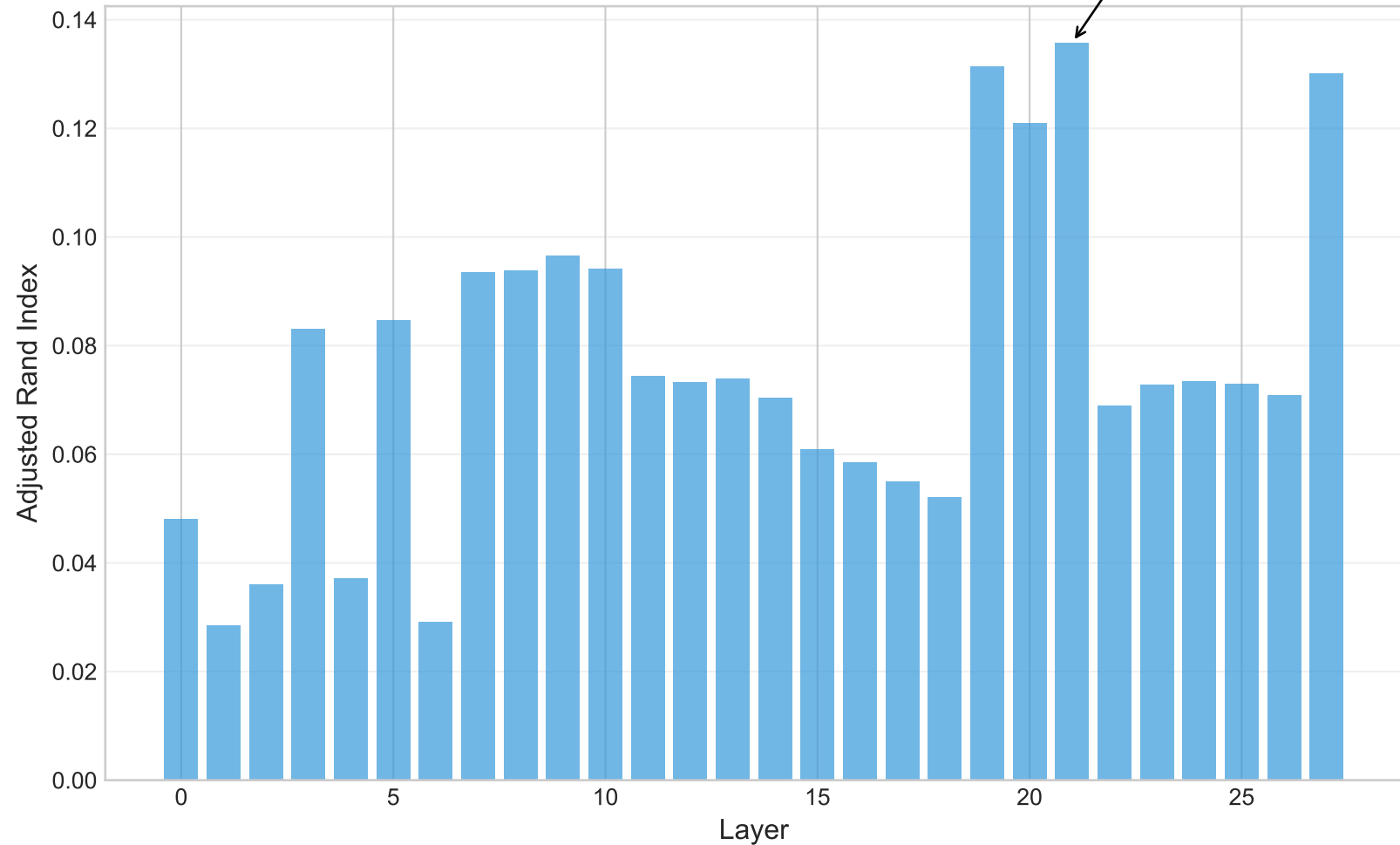
(qwen-2.5-7b) Clustering Quality (ARI) Across Layers
