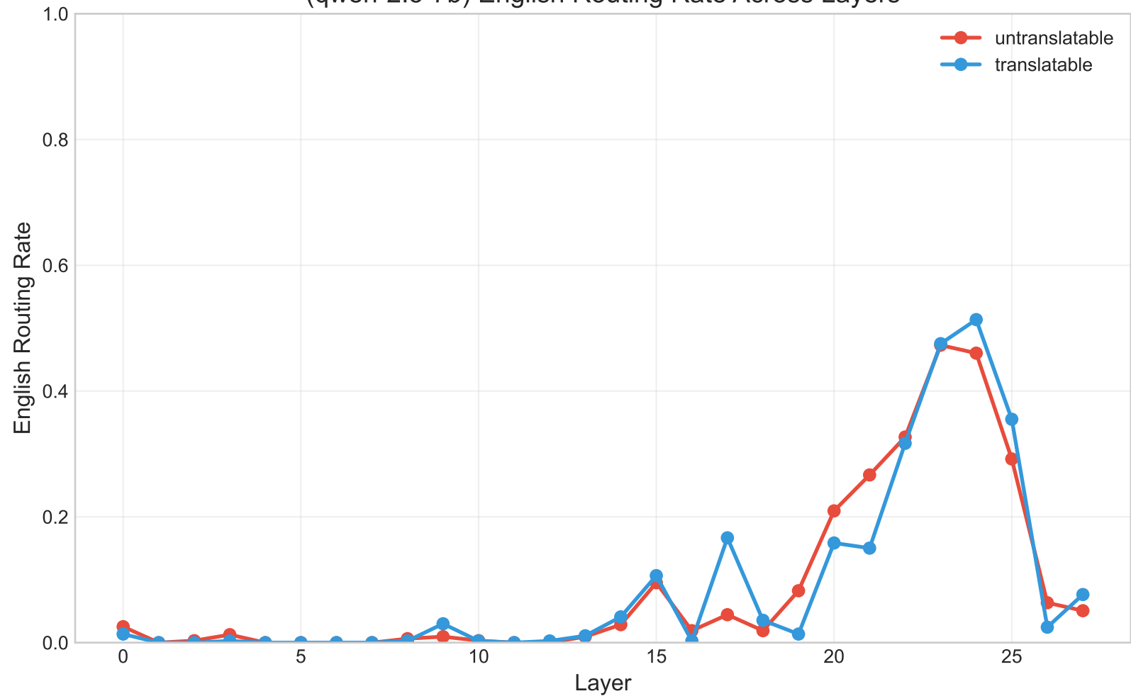
(qwen-2.5-7b) English Routing Rate Across Layers
