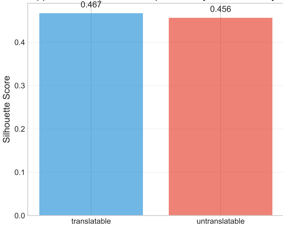
(qwen-2.5-7b) Cluster Separation by Translatability
