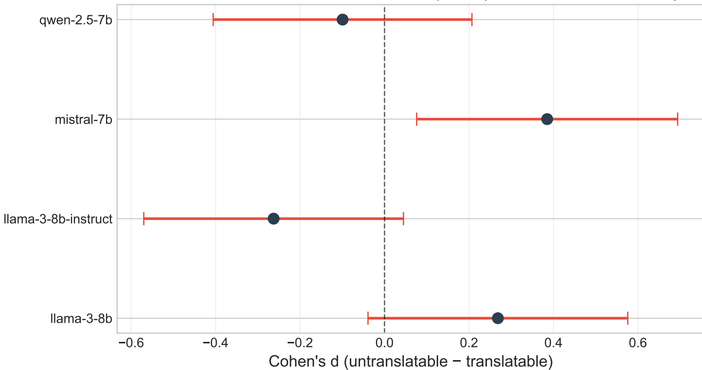
Faithfulness effect size on matched pairs (Cohen's d with 95% CI)
