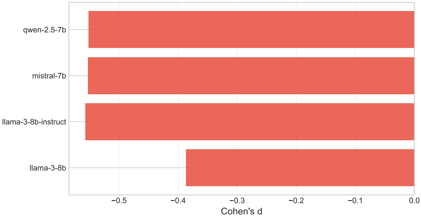
Faithfulness effect size (Cohen's d, untrans – trans)
