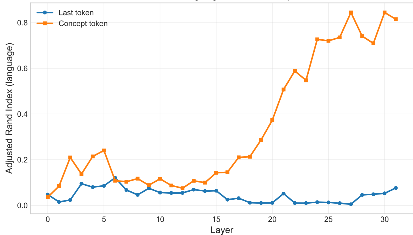
llama-3-8b-instruct: language ARI at concept vs last token
