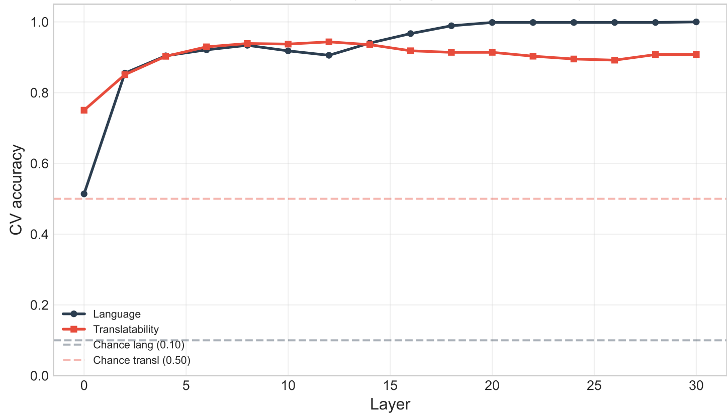
llama-3-8b (concept_token): language vs translatability probes
