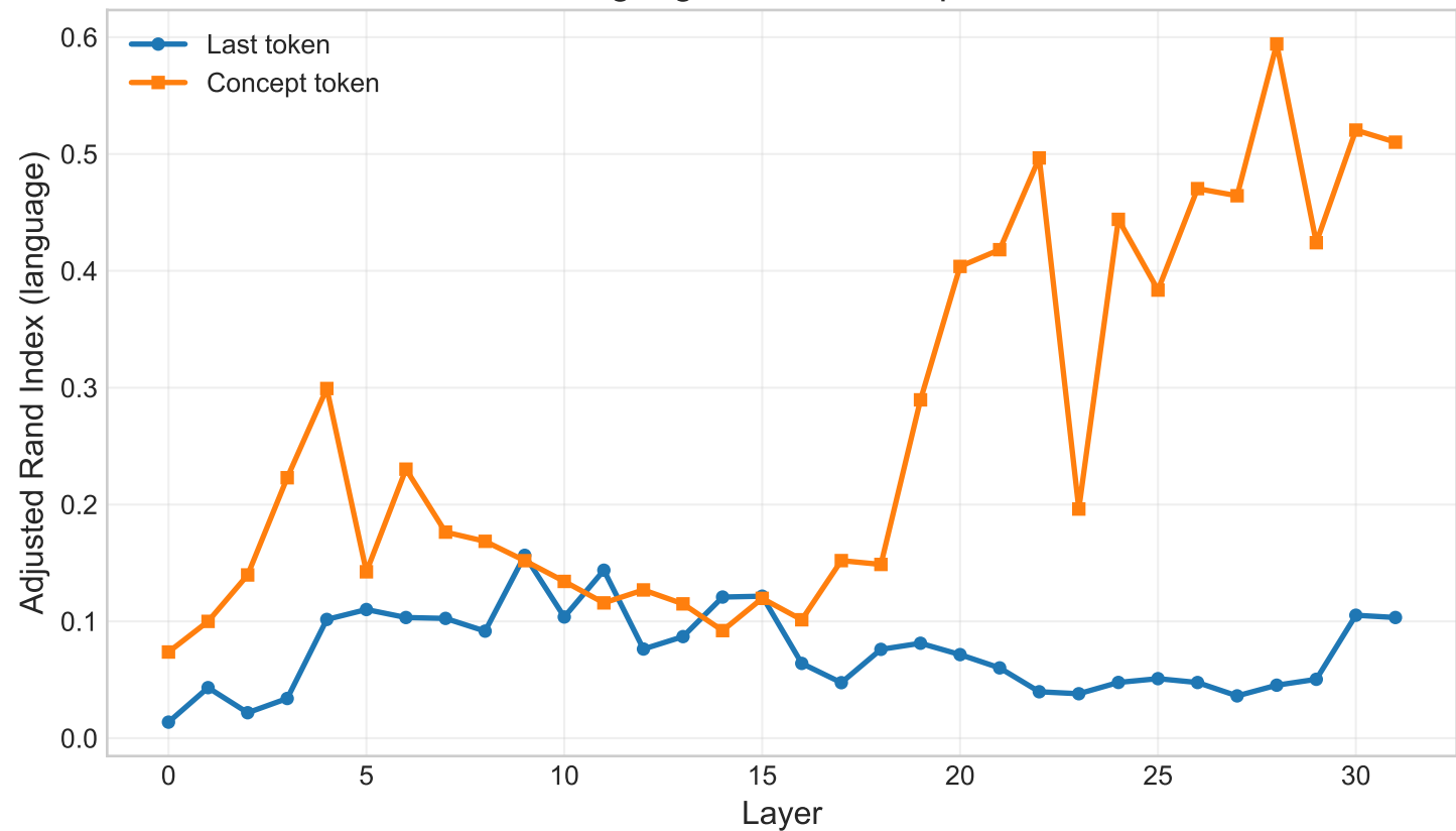
mistral-7b: language ARI at concept vs last token
