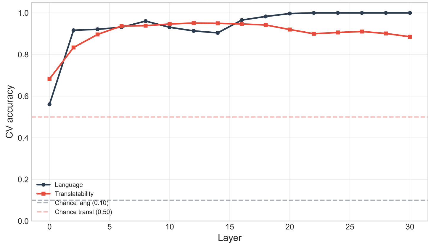
mistral-7b (concept_token): language vs translatability probes
