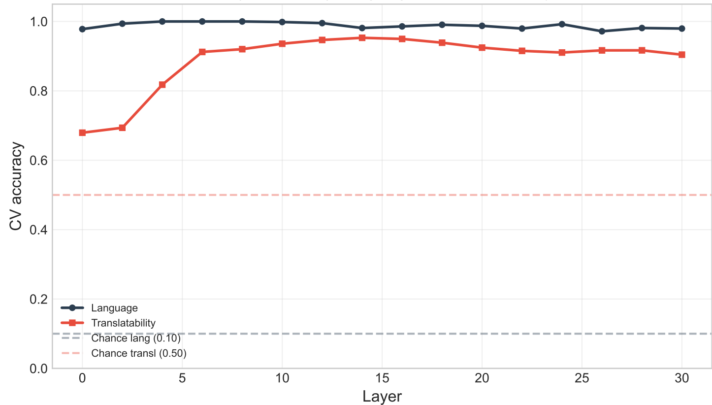
mistral-7b (last_token): language vs translatability probes
