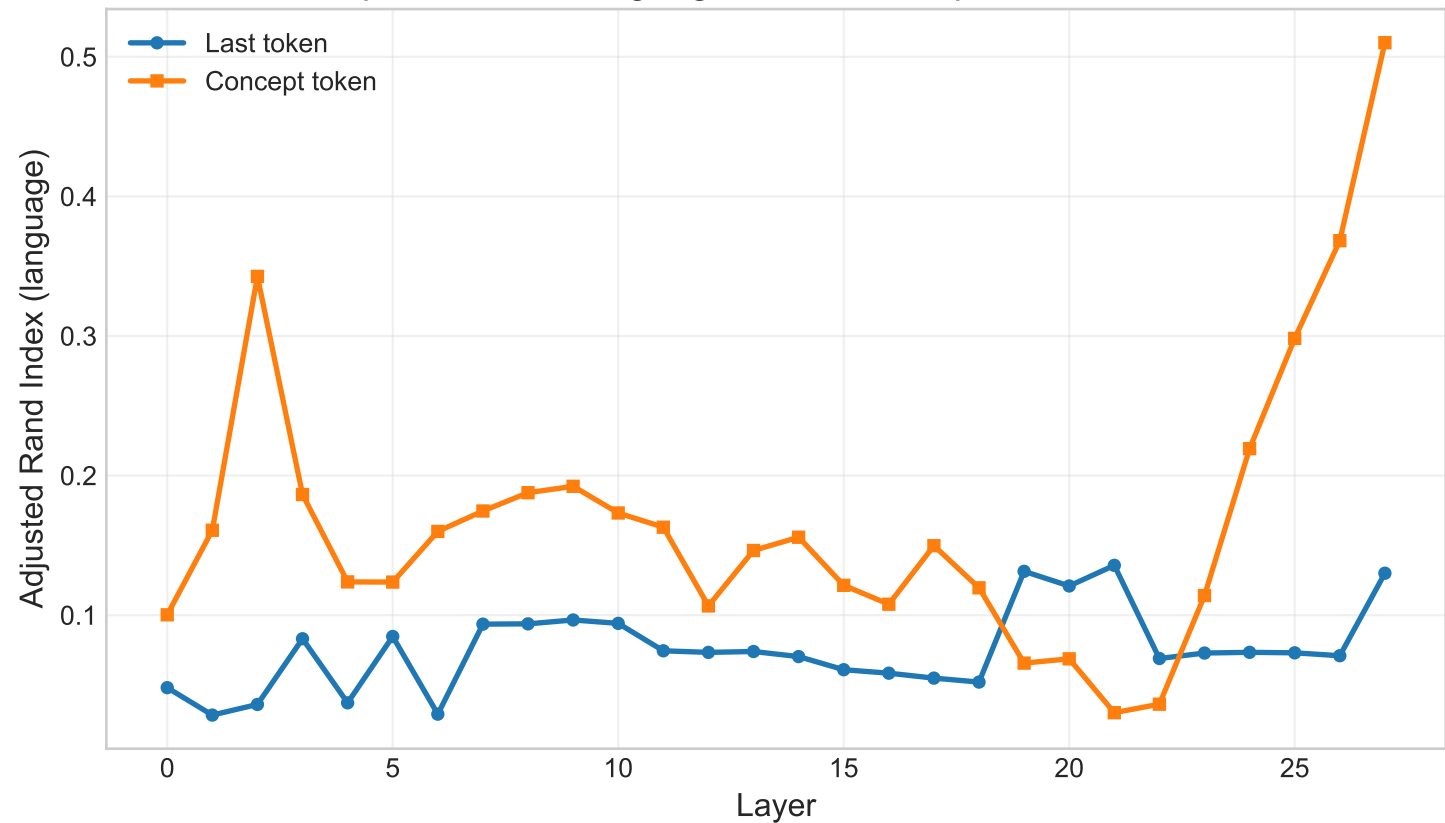
qwen-2.5-7b: language ARI at concept vs last token
