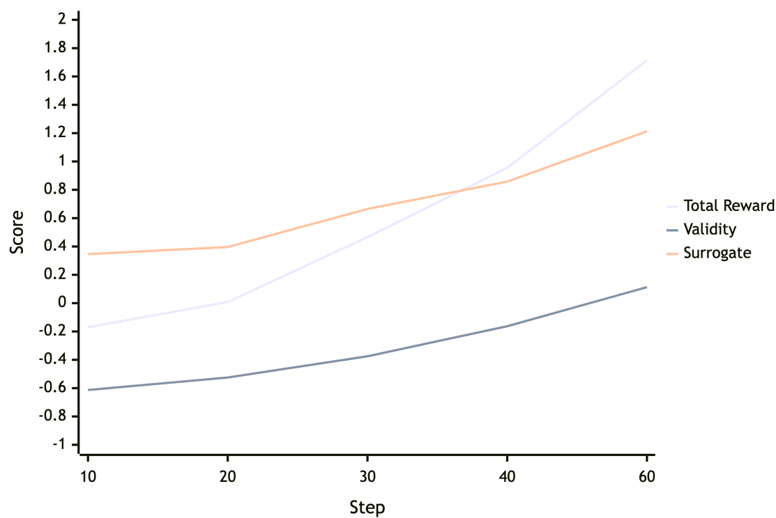
Qwen 0.5B – Reward Progression (60 steps)
