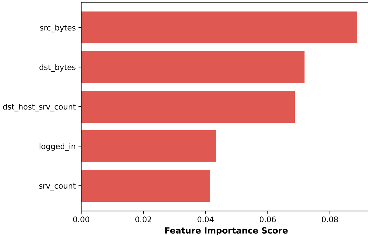
SHAP Explanation (Global Feature Importance)
