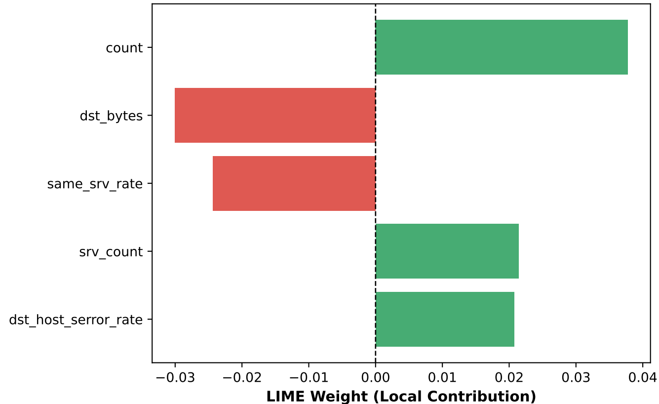
LIME Explanation (Local Interpretable Rules)
