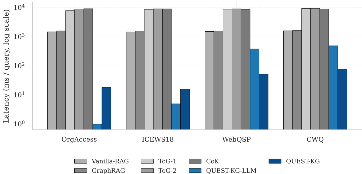
Inference latency: QUEST-KG is 19× to 500× faster than LLM baselines
