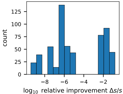
training data: 53056 logged (state, move, outcome) records
