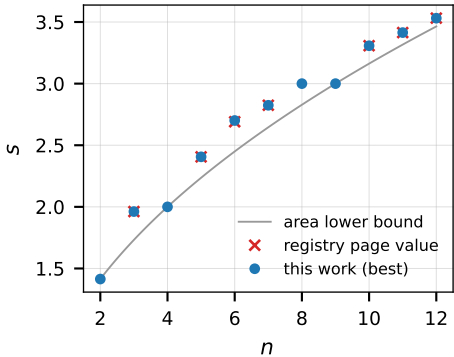
tans in tans
