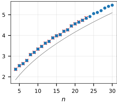
triangles in tans
