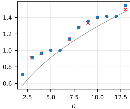
tans in L's
