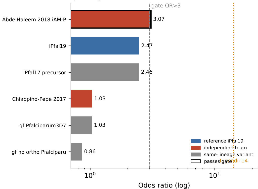
Fig 5B. Six P. falciparum GEMs (same organism+screen) span the gate: it sits at Plasmodium's noise floor
