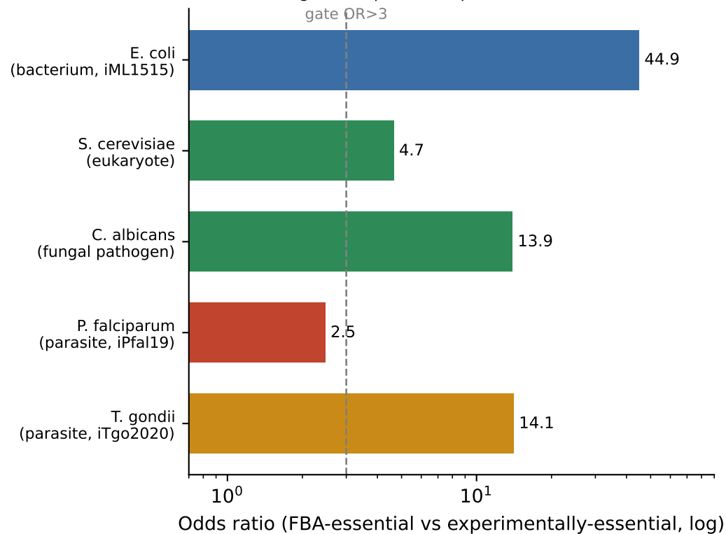
Fig 5A. FBA-essentiality transfers across classes — but is GEM/organism-specific for parasites
