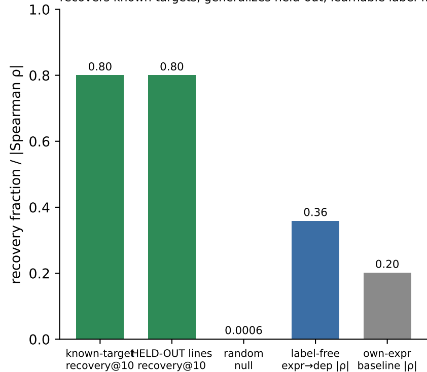
Fig 7A. Functional-dependency target-ID (DepMap): recovers known targets, generalizes held-out, learnable label-free
