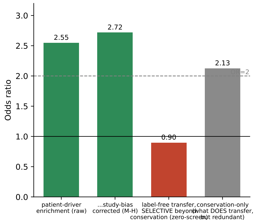
Fig 7B. Patient relevance is REAL (survives study-bias), but label-free transfer to a novel organism is NOT (a first-class negative)
