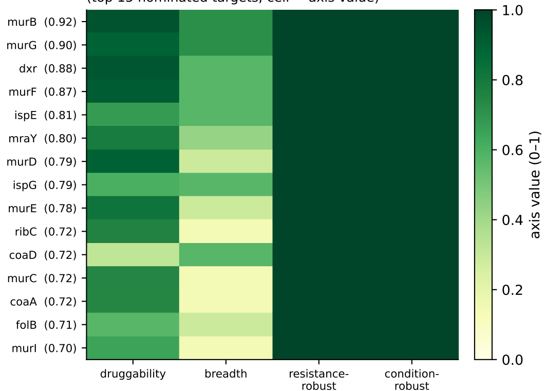
Fig 4a. Multi-axis best-intervention scorecard (top 15 nominated targets; cell = axis value)
