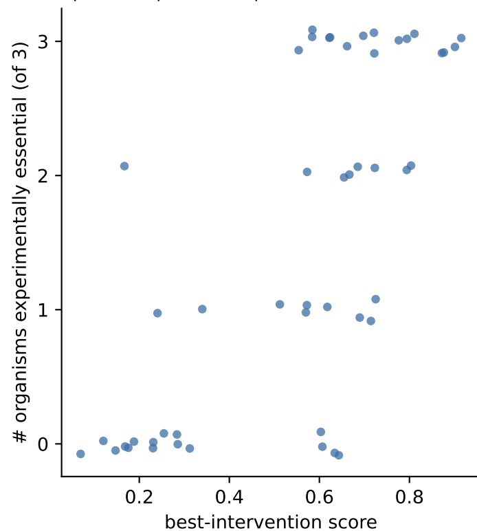
Fig 4b. Score vs experimental essentiality Spearman \rho=0.6896 , p=0.0 ( n=49 )
