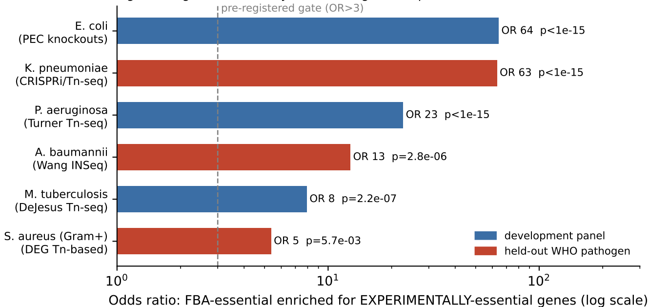
Fig 1. FBA gene-essentiality validated against experimental knockout data in 6 bacteria (incl. Gram-positive)
