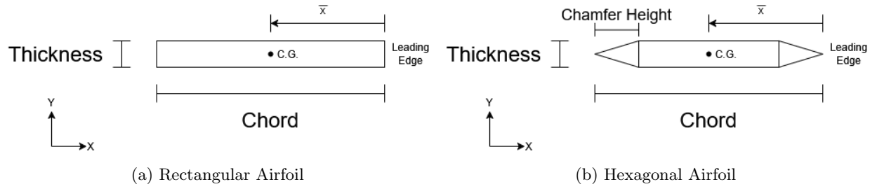
Figure 2: Airfoil dimensions for rectangular and hexagonal fins
