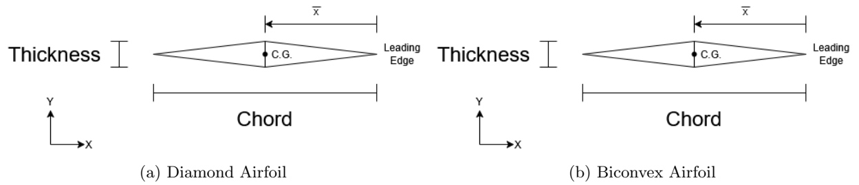
Figure 3: Airfoil dimensions for diamond and biconvex fins
