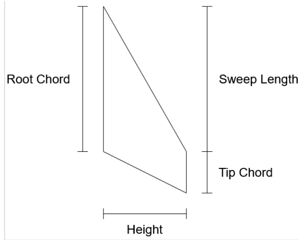
Figure 1: Fin Planform Dimensions
