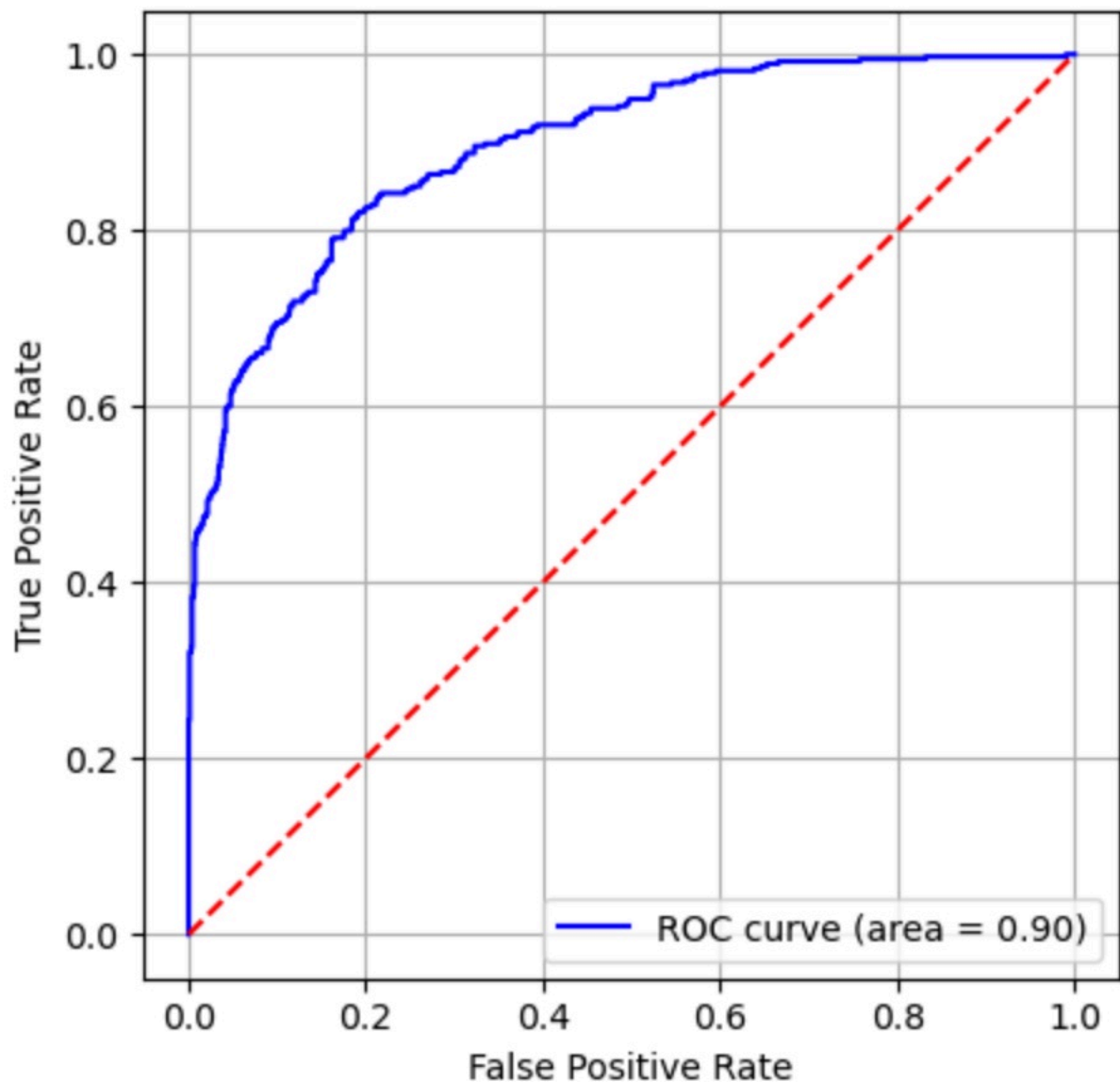
Receiver Operating Characteristic (ROC) Curve for XGBoost model with "test" dataset
