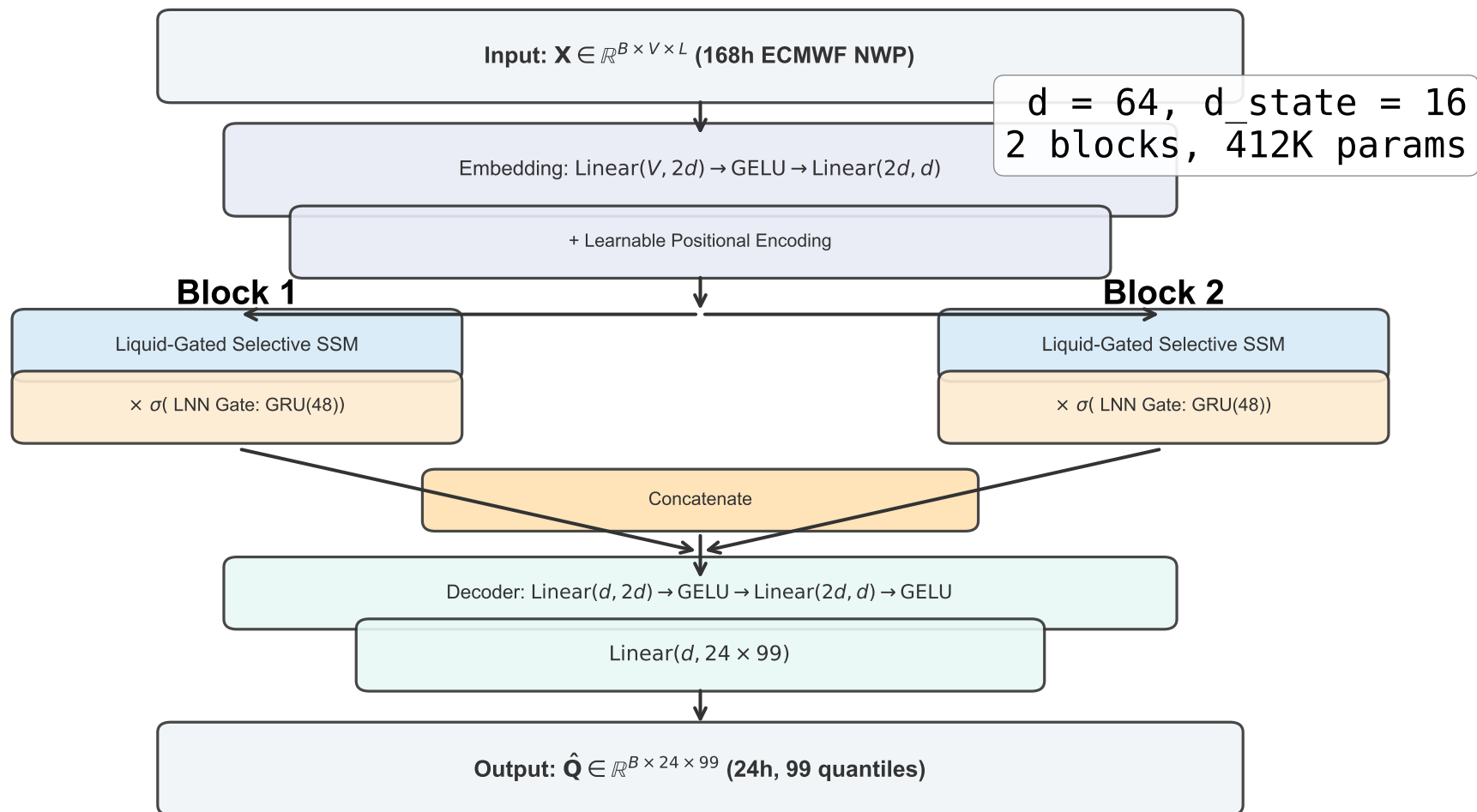
Figure 1: LNMamba Architecture
