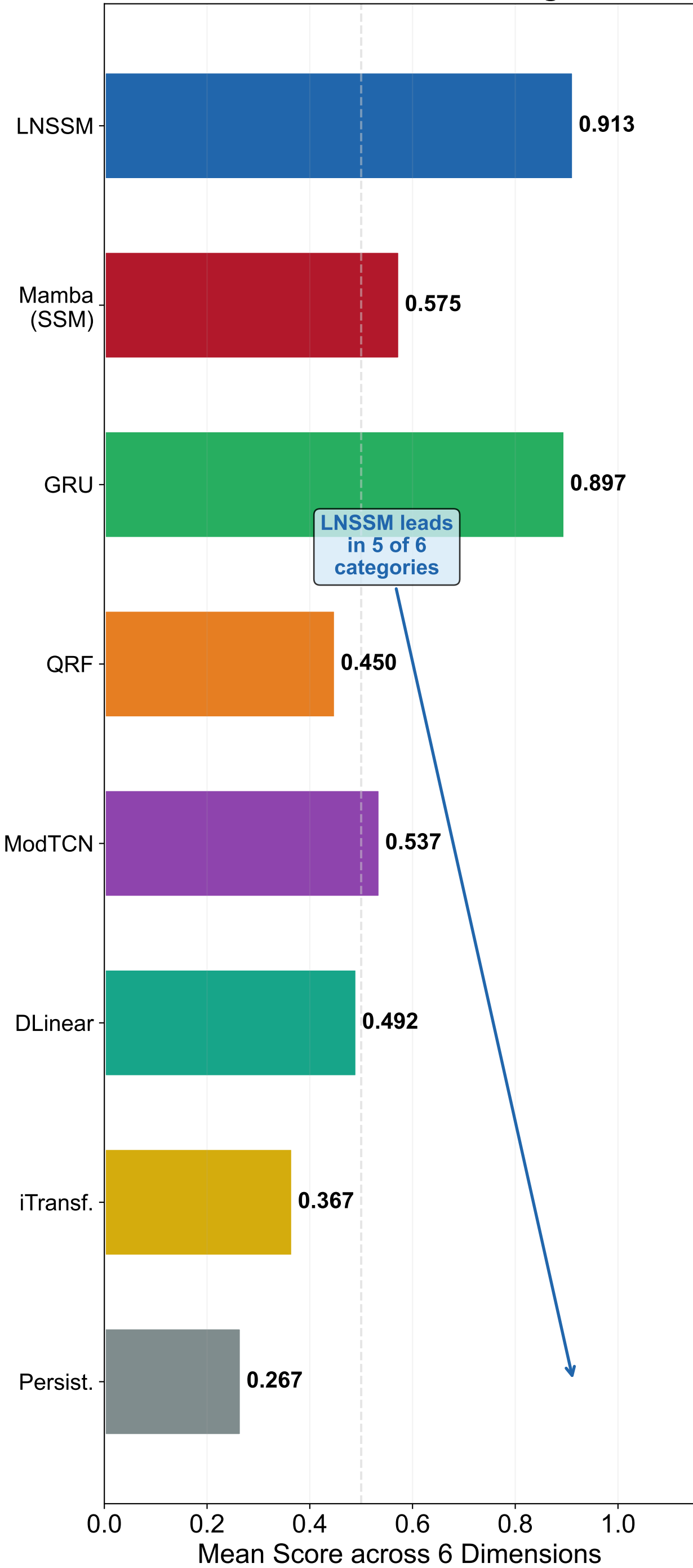
Overall Score Ranking
