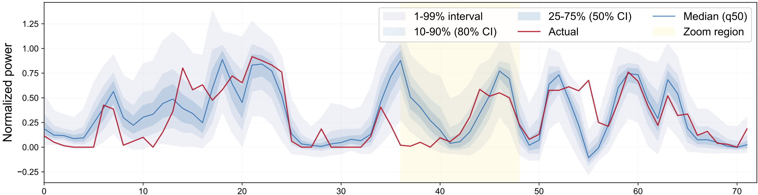
Zoom (12h) — 50% captured in 80% CI
