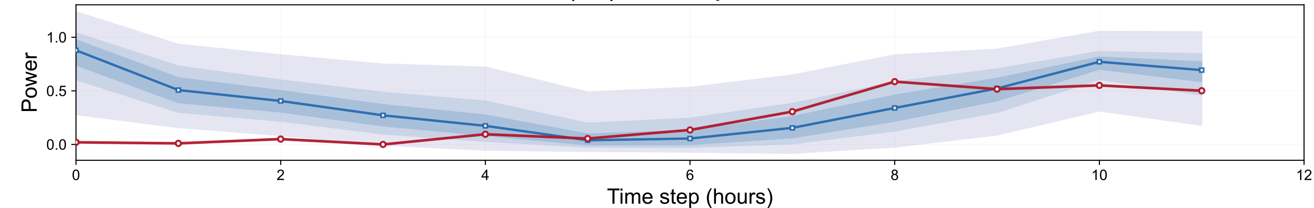
Zoom (12h) — 50% captured in 80% CI
