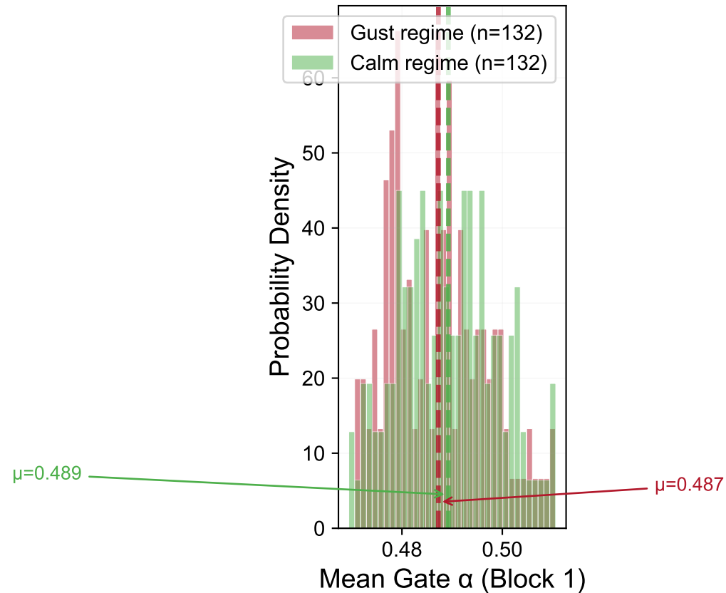
Gust vs Calm regimes KS D=0.129, p=0.2242
