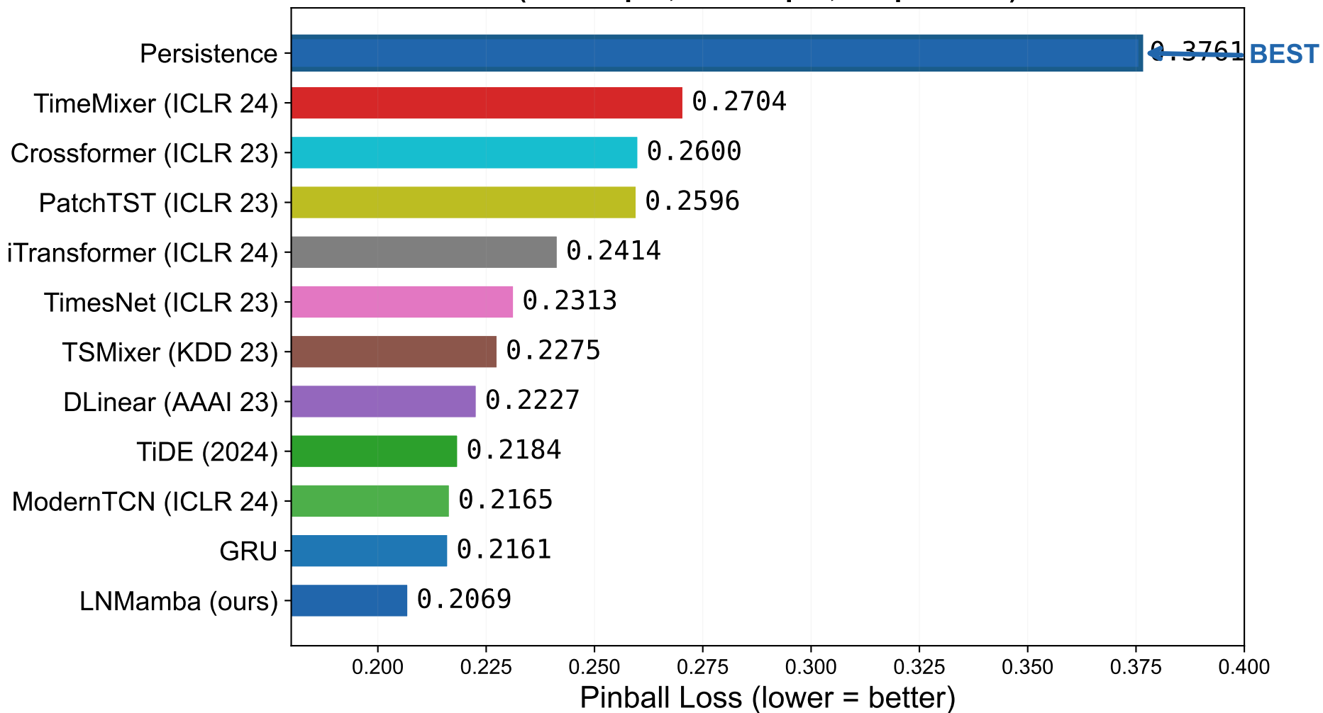
Figure 2: SOTA Comparison — 12 Models on GEFCom2014 Zone 1 (168h input, 24h output, 99 quantiles)
