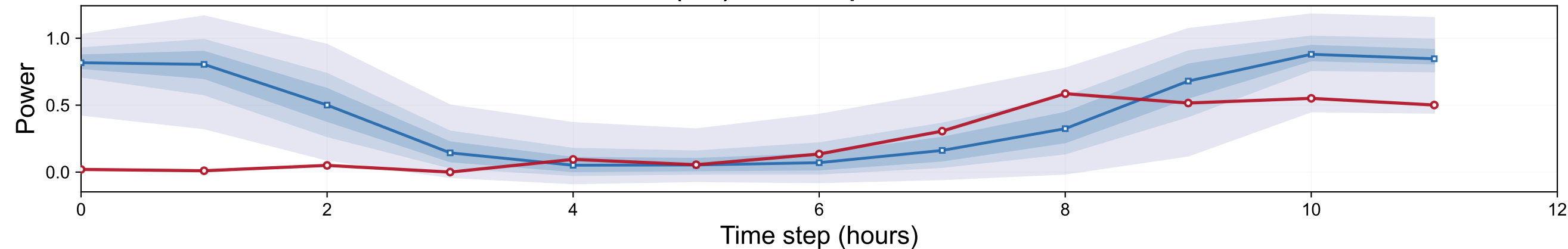
Zoom (12h) — 42% captured in 80% CI
