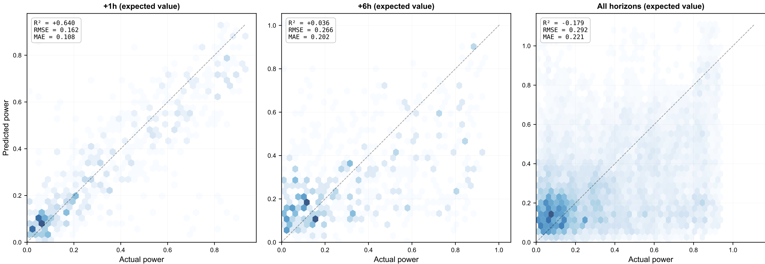
Figure 2: Point Forecast Accuracy — Predicted vs Actual Wind Power
