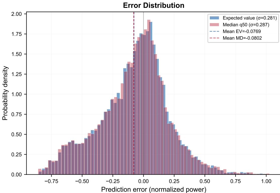
Figure 6: Prediction Error Analysis
