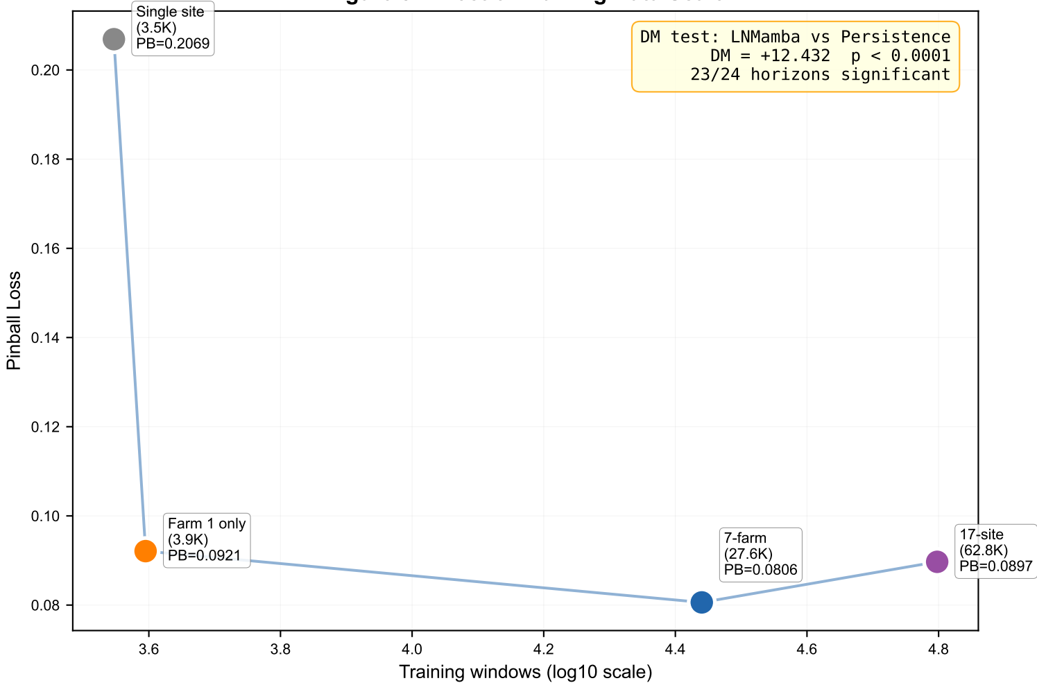
Figure 8: Effect of Training Data Scale
