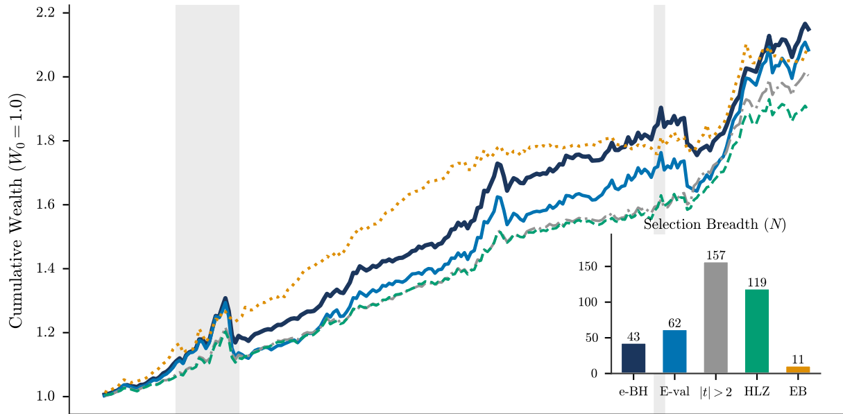
Panel A: Cumulative Out-of-Sample Performance of Factor-Screening Portfolios (2006--2023)
