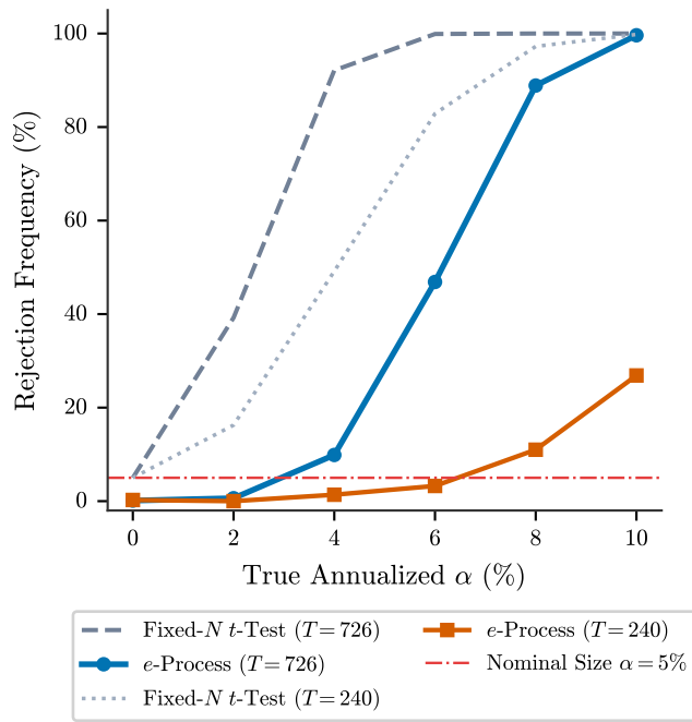
Panel A: Empirical Power Trade-Off across Sample Size and Horizontal Empirical Size under Heavy-Tailed Residual DGPs
