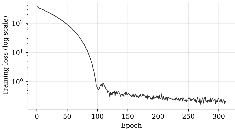
Deep BSDE training loss ( \theta = 0.4 )
