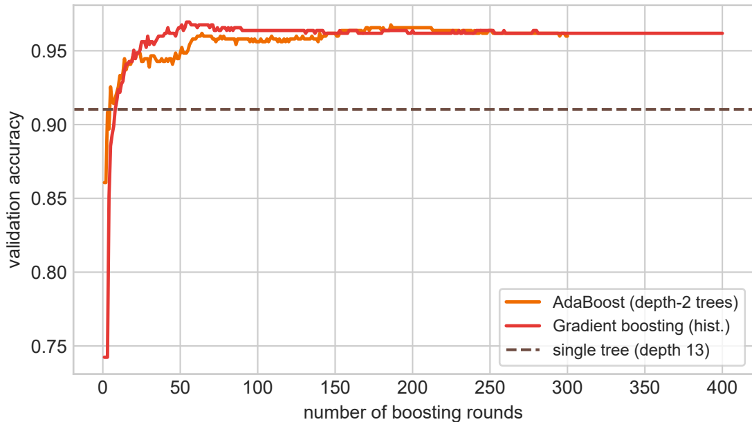
Boosting improves on a single tree
