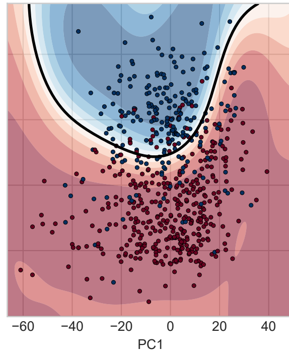
RBF-SVM (test acc. in 2D = 0.824)
