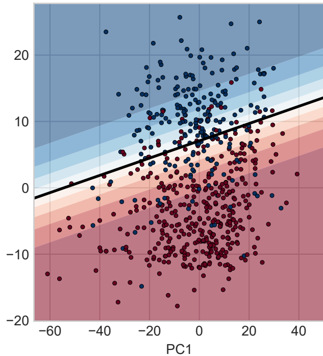
Logistic regression (test acc. in 2D = 0.835)
