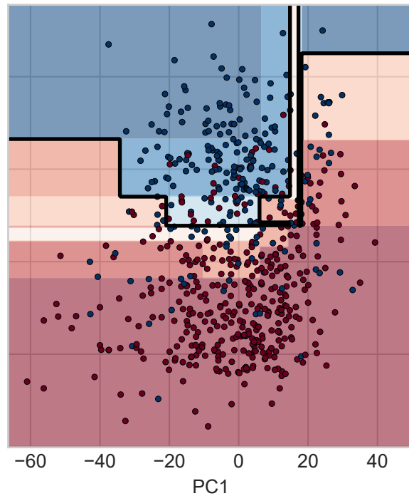
Decision tree (depth 5) (test acc. in 2D = 0.819)
