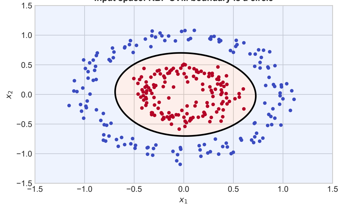
Input space: RBF-SVM boundary is a circle
