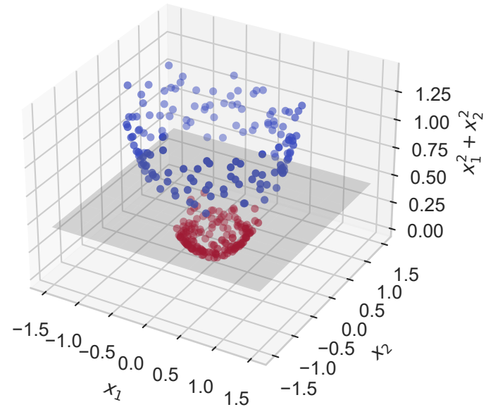
Feature space \varphi(x) = (x_1, x_2, x_1^2 + x_2^2) : a plane separates
