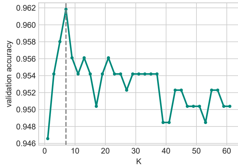
Role of K
