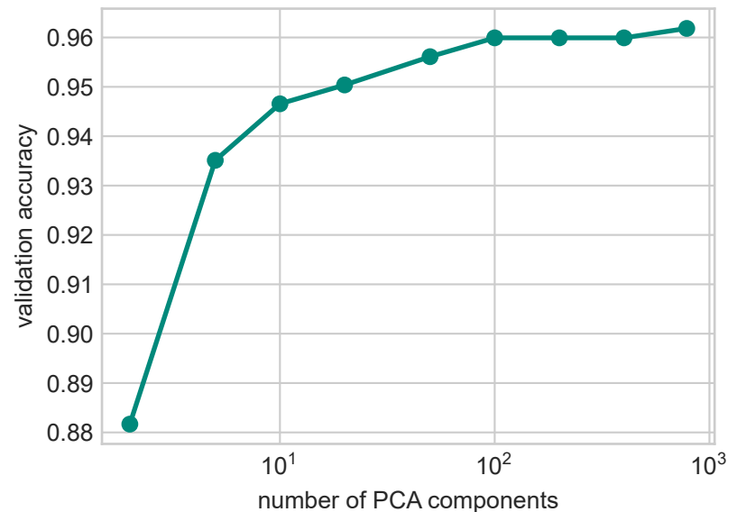
KNN (K=7) vs dimension
