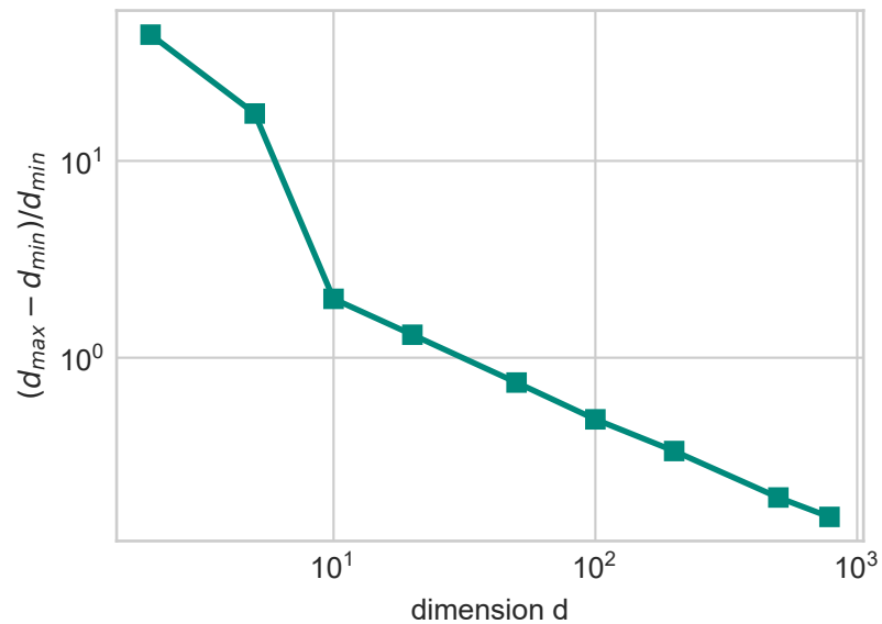
Distance concentration (uniform data)
