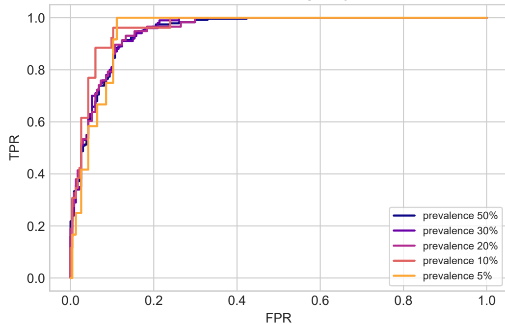
ROC of RBF-SVM: unchanged by prevalence
