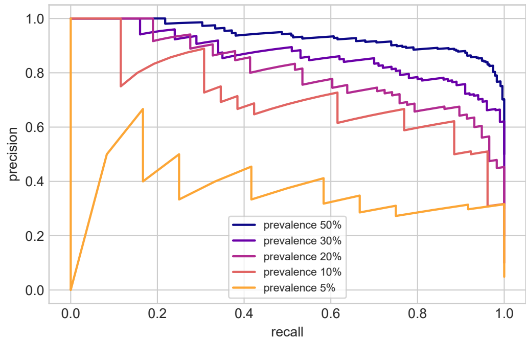
PR of RBF-SVM: collapses when disease is rare
