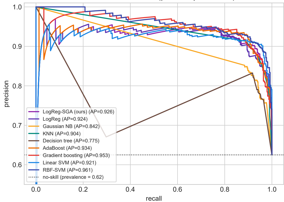
Precision-Recall curves (positive: pneumonia)
