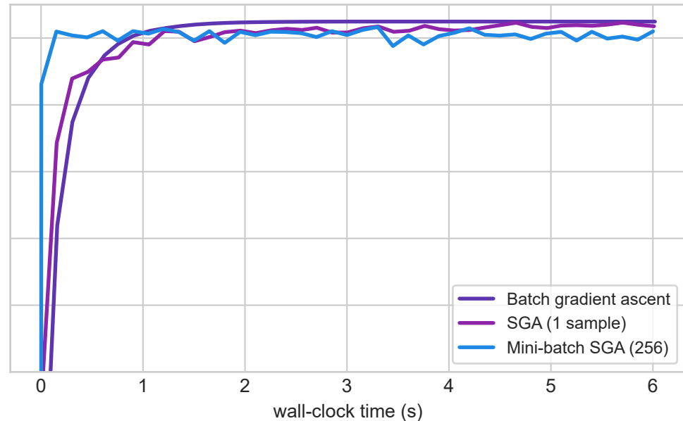
Computational efficiency (NumPy)
