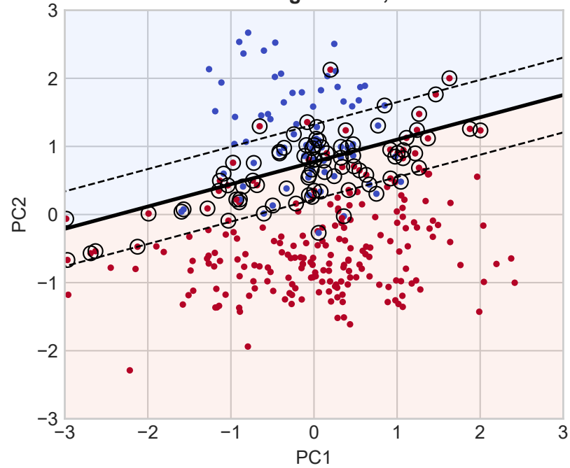
C = 100: margin = 1.05, 91 SVs
