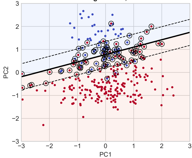
C = 1: margin = 1.08, 94 SVs
