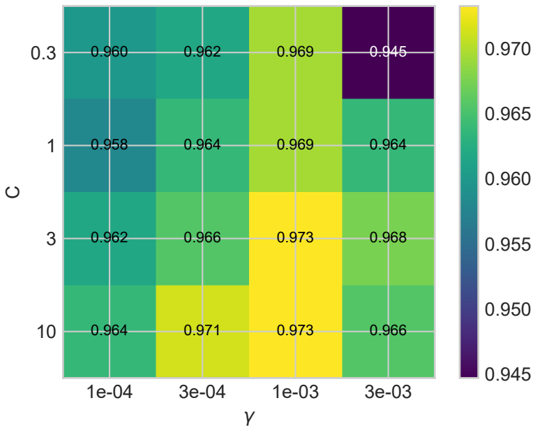
RBF-SVM validation accuracy
