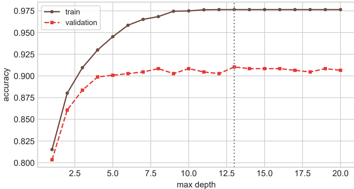
Decision tree: depth vs over-fitting
