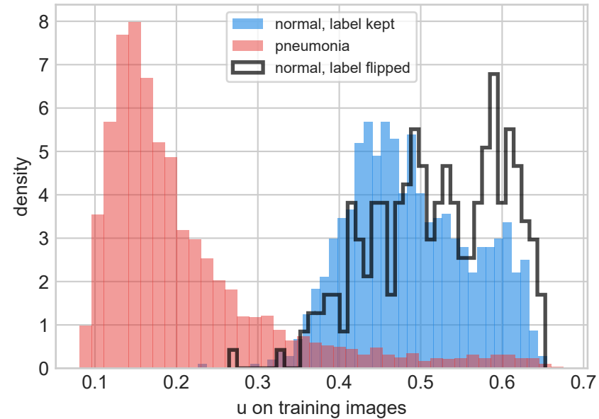
EDL trained with 20% flipped labels
