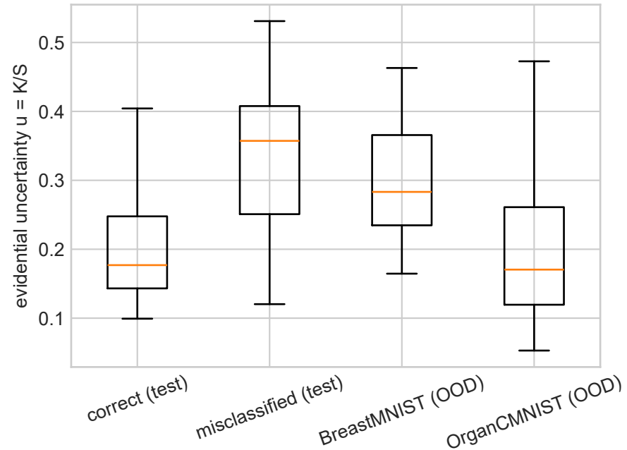
EDL uncertainty (clean training)
