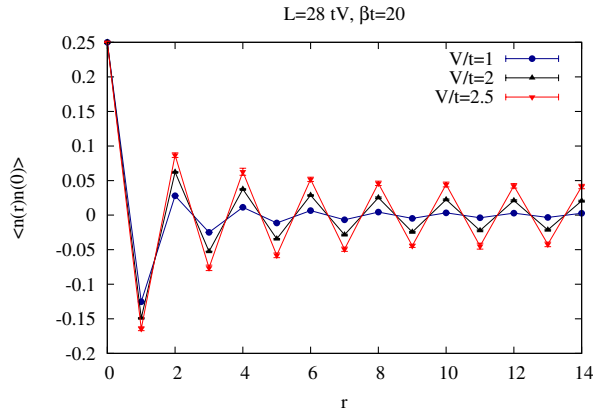
Figure 2: Density-Density correlation functions of the t-V model. In the Luttinger liquid phase, -2 < V/t < 2 it is known that the density -density correlations decay as \langle n(r)n(0) \rangle \propto \cos(\pi r) r^{-(1+K_\rho)} with (1+K_\rho)^{-1} = \frac{1}{2} + \frac{1}{\pi} \arcsin\left(\frac{V}{2|t|}\right) (A. Luther and I. Peschel, Calculation of critical exponents in two dimensions from quantum field theory in one dimension, Phys. Rev. B 12 (1975), 3908.) The interested reader can try to reproduce this result.
