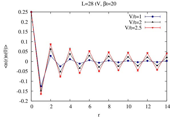
Figure 3: Density-Density correlation functions of the t-V model. In the Luttinger liquid phase, -2 < V/t < 2 it is known that the density -density correlations decay as \langle n(r)n(0) \rangle \propto \cos(\pi r) r^{-(1+K_\rho)} with (1 + K_\rho)^{-1} = \frac{1}{2} + \frac{1}{\pi} \arcsin\left(\frac{V}{2|t|}\right) (A. Luther and I. Peschel, Calculation of critical exponents in two dimensions from quantum field theory in one dimension, Phys. Rev. B 12 (1975), 3908.) The interested reader can try to reproduce this result.
