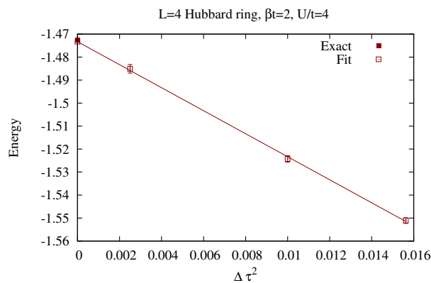
Figure 1: \Delta\tau t extrapolation for the 4-site Hubbard ring.
