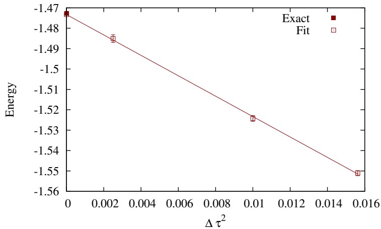
L=4 Hubbard ring, \beta t=2 , U/t=4
