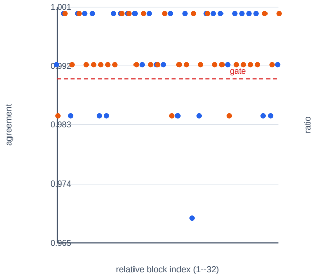
Top-1 agreement by block
