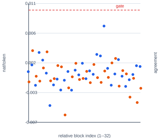
Delta NLL by block
