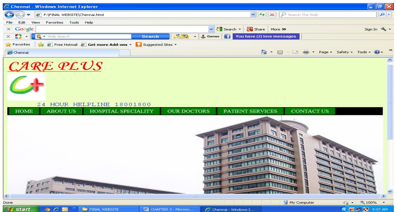
Figure 3.26: “Chennai” page
