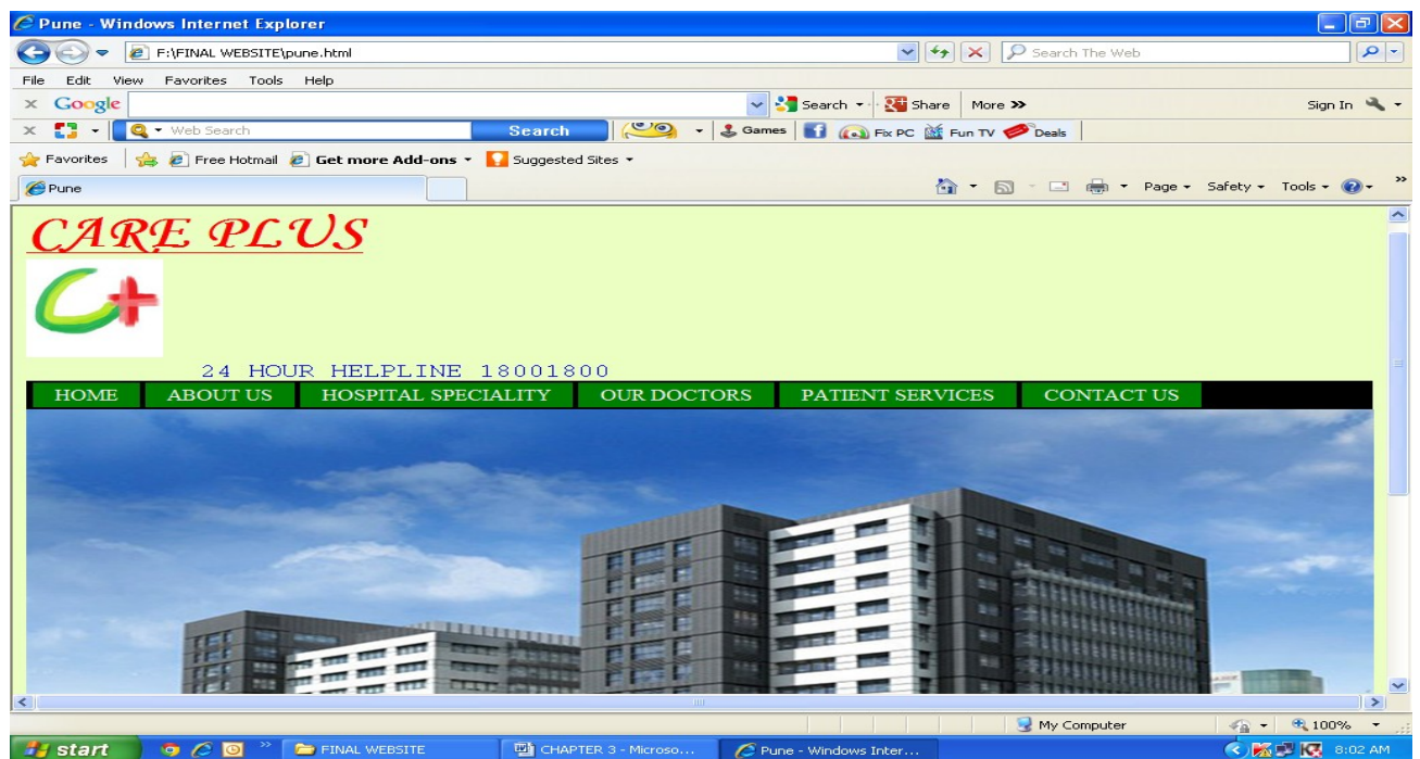
Figure 3.23 : “pune” page
