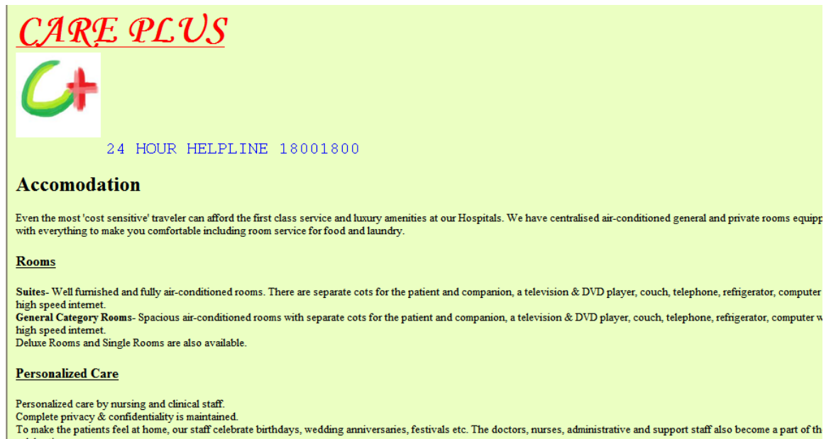
Figure 3.16 : “accommodation & facilities”page
