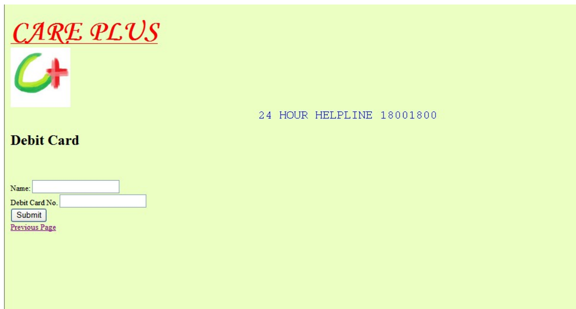
Figure 3.18.2 : “debit card”page
