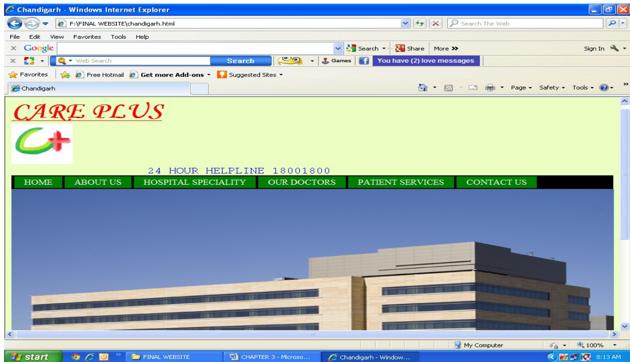
Figure 3.29 : “Chandigarh” page
