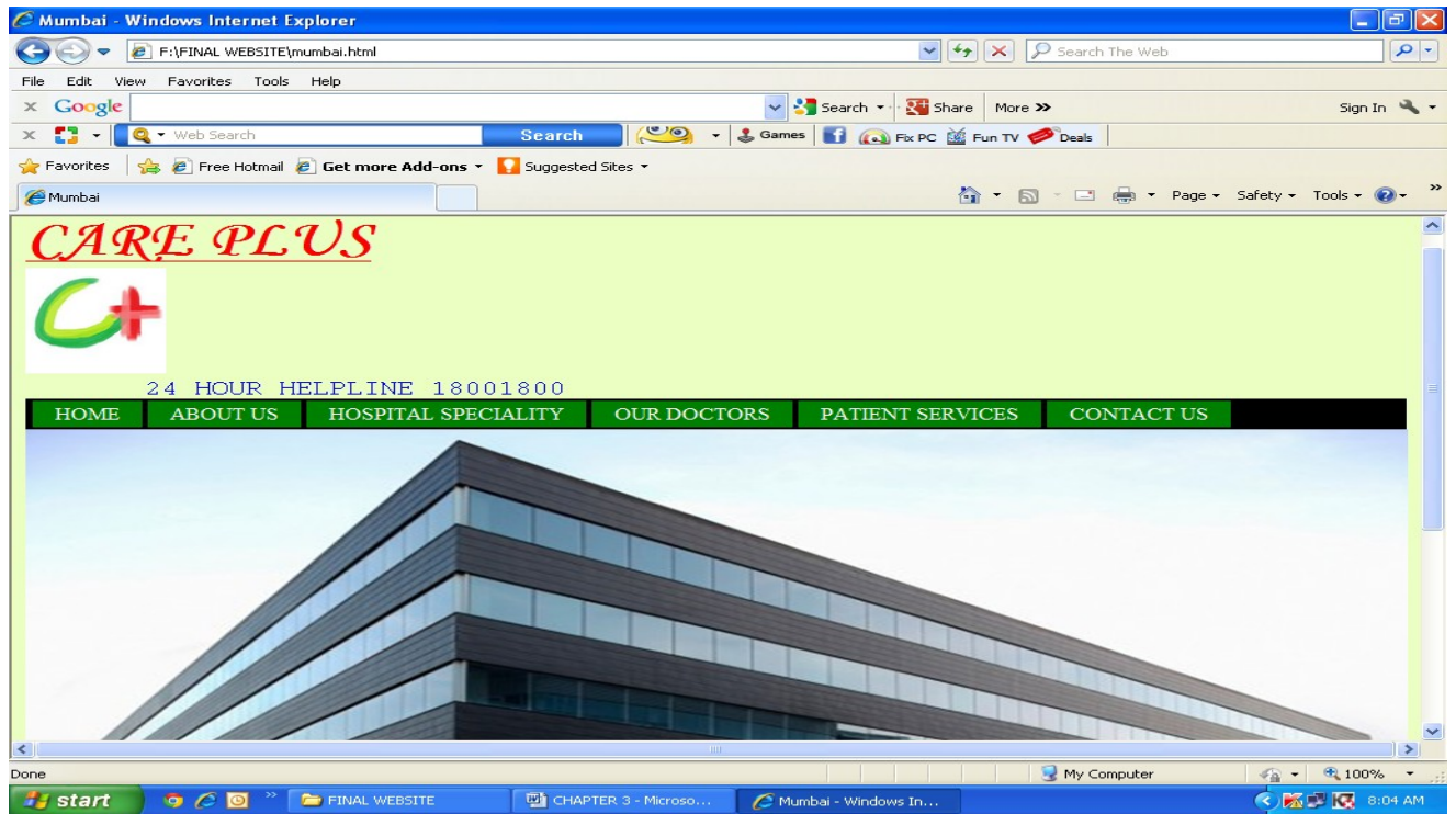
Figure 3.24 : “mumbai” page
