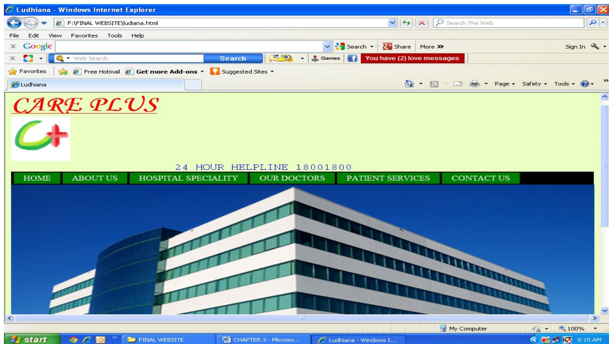
Figure 3.30: “Ludhiana” page
