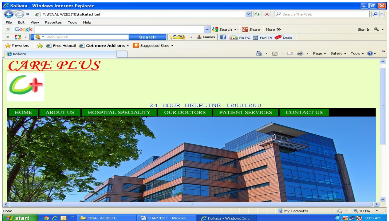
Figure 3.25: “Kolkata” page
