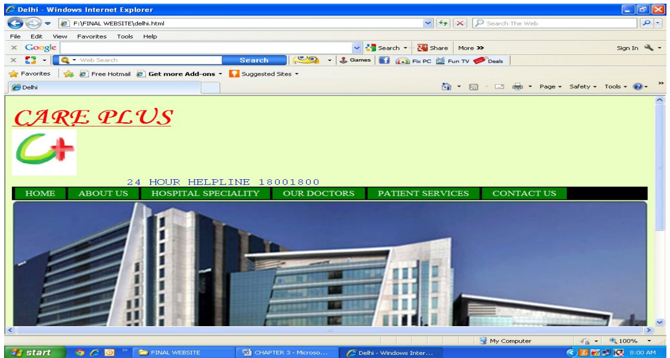
Figure 3.22 : “delhi” page
