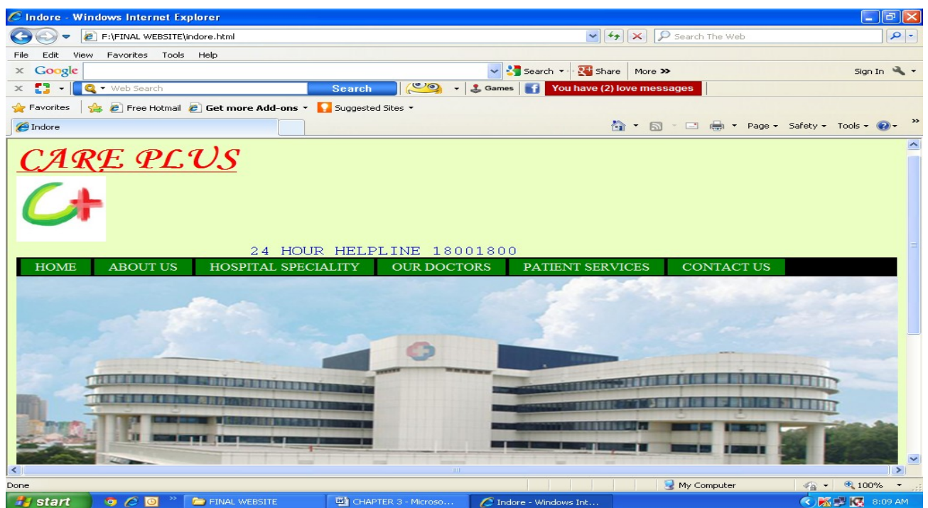
Figure 3.27: “indore” page
