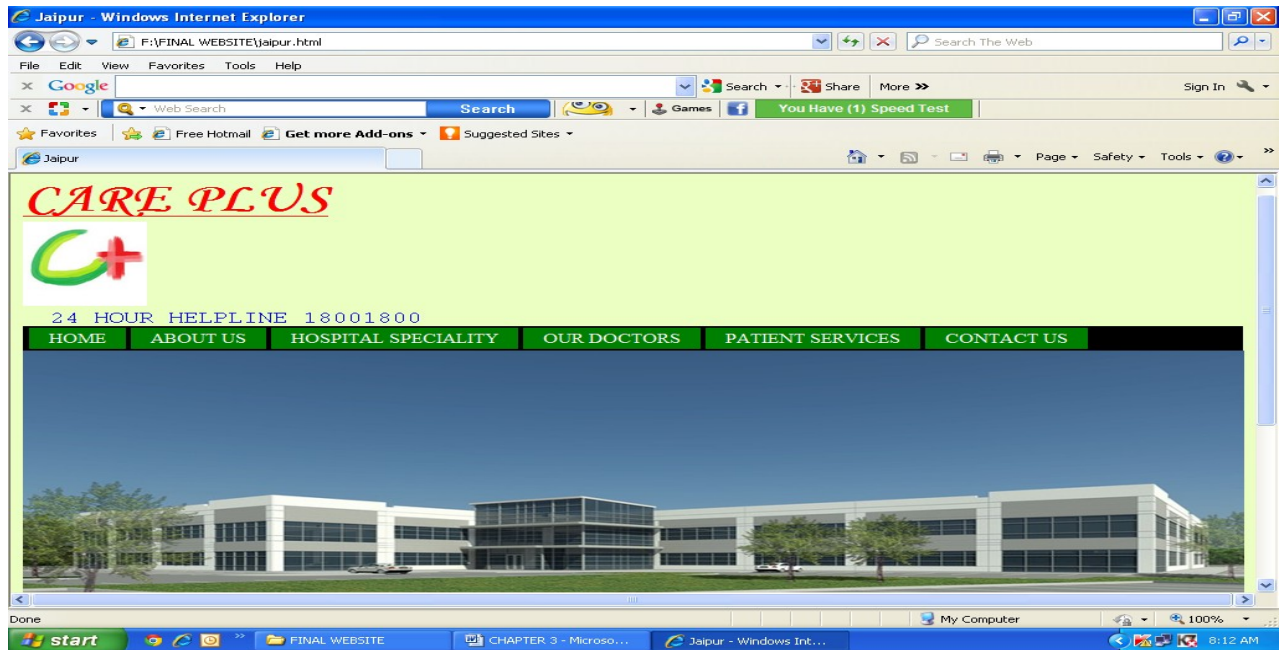
Figure 3.28: “jaipur” page
